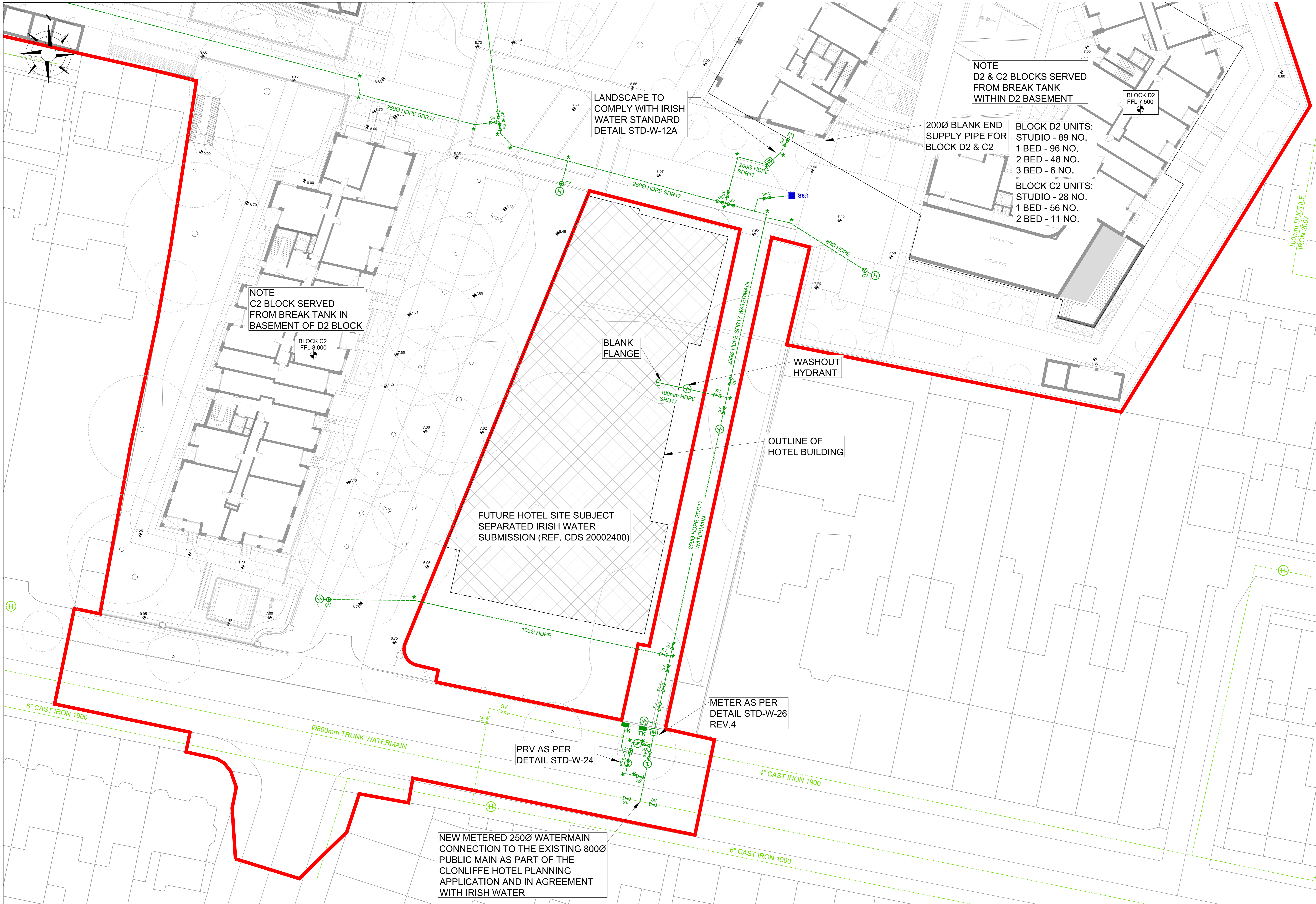
PROPOSED WATERMAIN SITE PLAN LAYOUT - SHEET 8 OF 8
